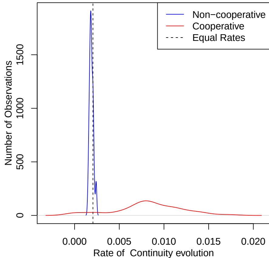
CoopBreed Continuity all converged runs from 2021-08-18CoopBreedContinuitybrownie500sim.csv
